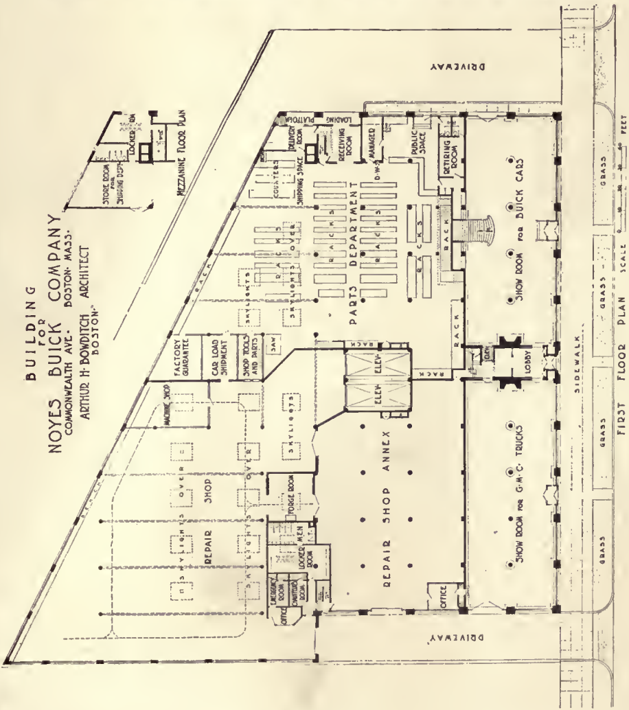
FLOOR PLANS NOYES-BUICK BUILDING, BOSTON, MASS. ARCHITUR H. BOWDITCH, ARCHITECT
